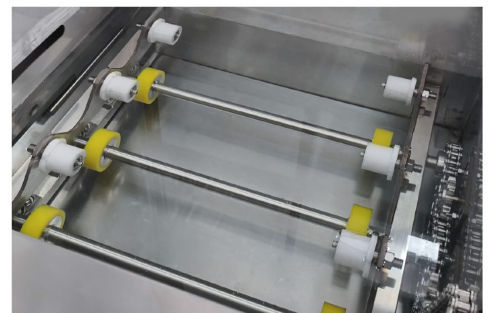
▲ Triple-Spindle Setup
