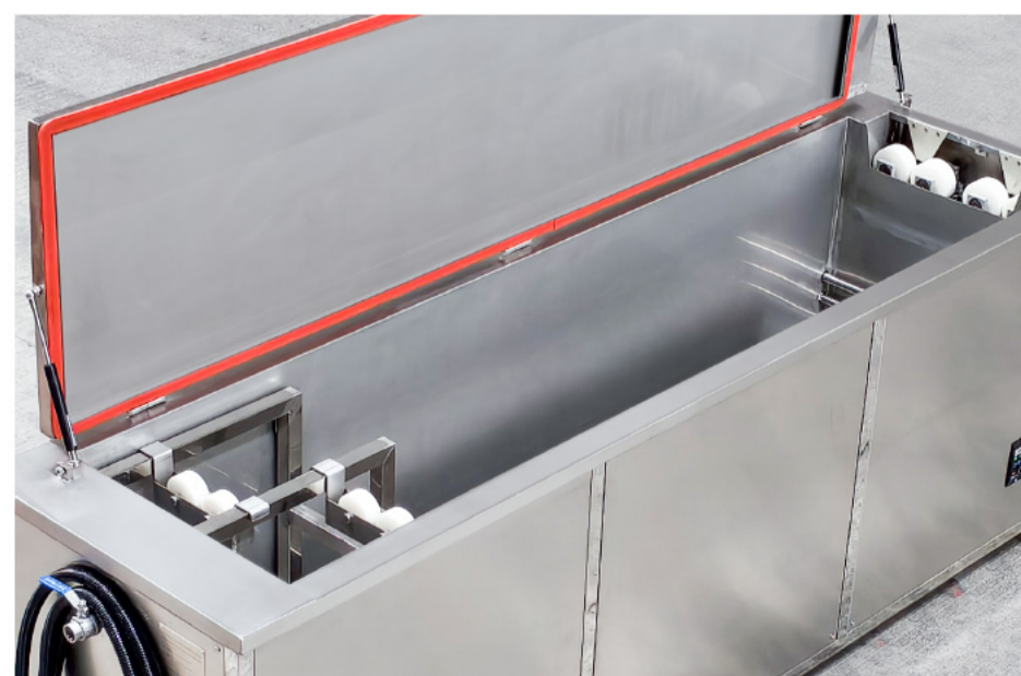
▲ Dual-Spindle Setup
